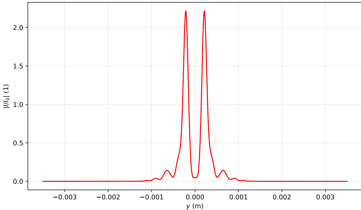
Intensity profile I(x=0, y, z=0.716)/I_0 , P_{in}=5.0P_{cr} , artificial time
